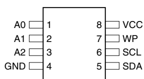
8-lead PDIP
