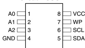
8-lead PDIP
