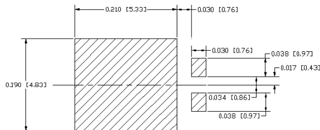
Mounting Pad Dimensions: inches [mm]
