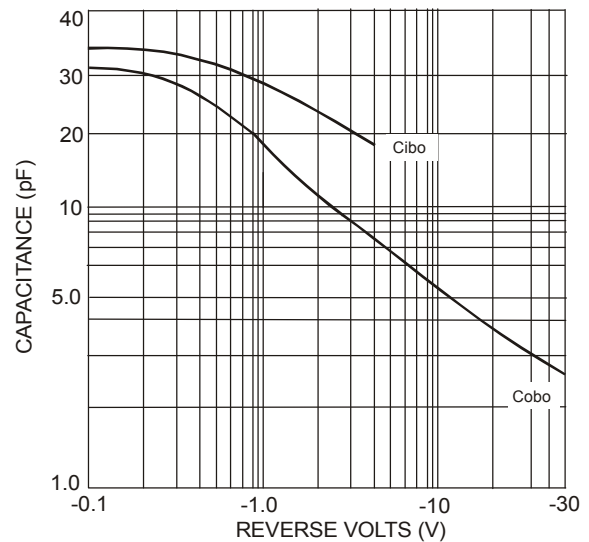
Fig. 2 Capacitances (Typical)
