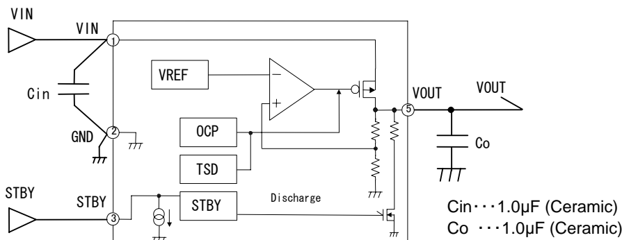
Fig. 2 Block Diagrams
