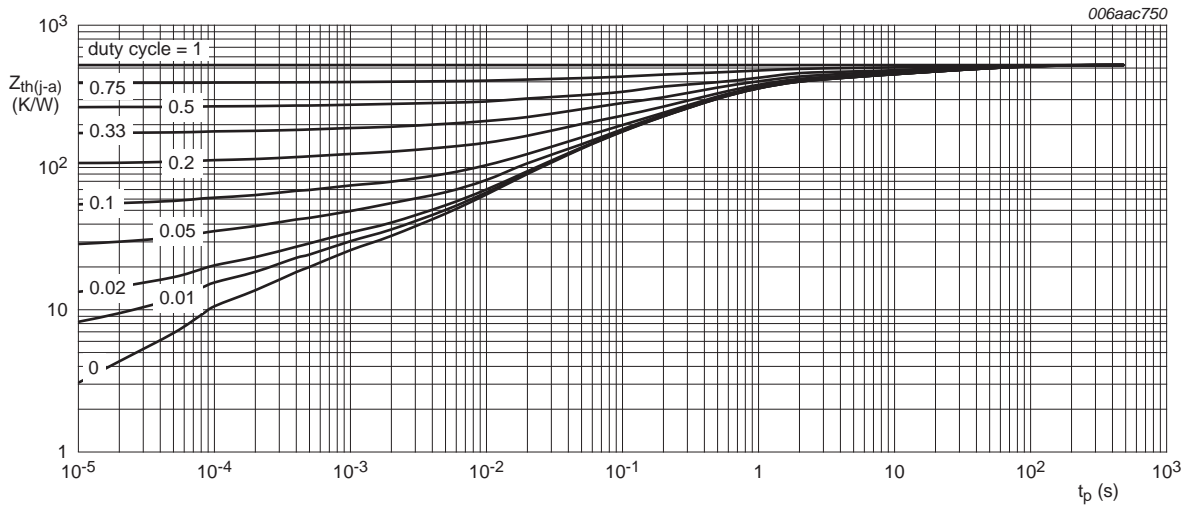
Fig 3. Per transistor: Transient thermal impedance from junction to ambient as a function of pulse duration for PUMH15 (SOT363); typical values
