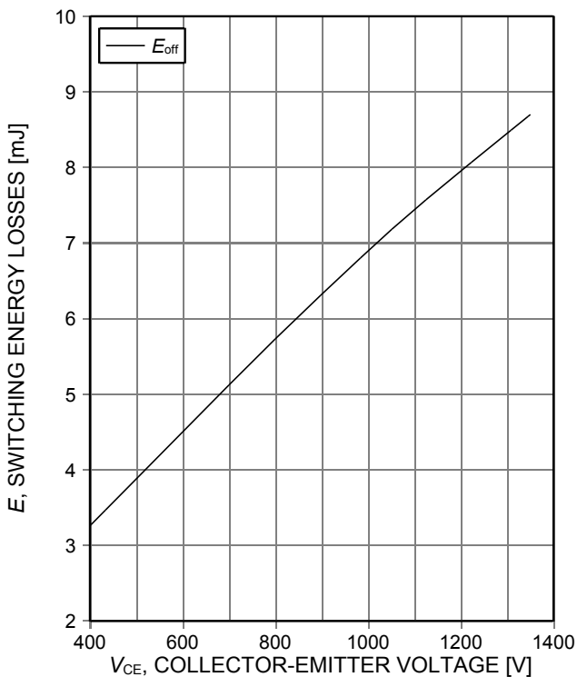
Figure 15. Typical switching energy losses as a function of collector emitter voltage (inductive load, T_{vj}=175^\circ\text{C} , V_{GE}=0/15\text{V} , I_C=40\text{A} , R_{G(on)}=7.5\Omega , R_{G(off)}=7.5\Omega , dynamic test circuit in Figure E)
