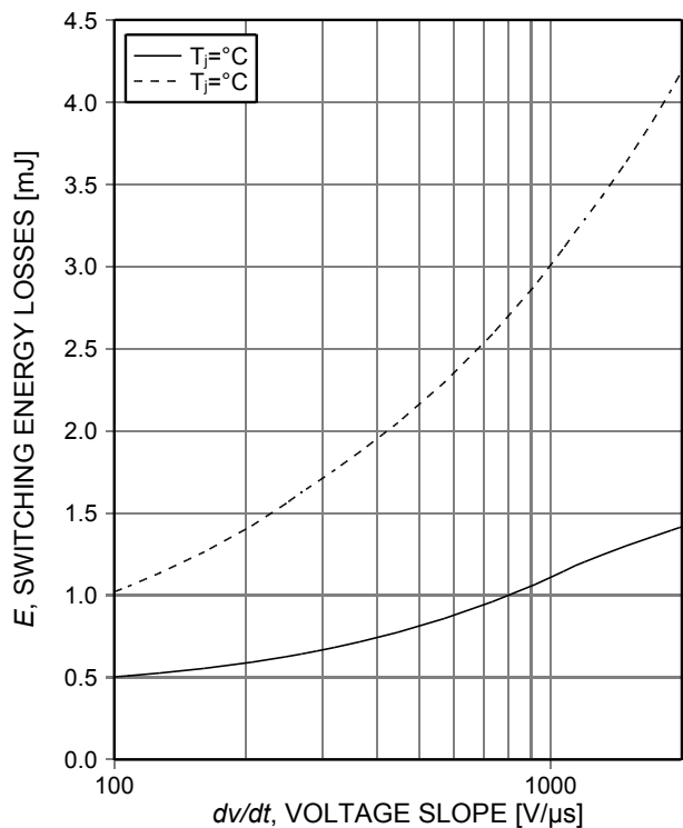
Figure 16. Typical turn off switching energy loss for soft switching (inductive load, T_{vj}=175^\circ\text{C} , V_{GE}=0/15\text{V} , I_C=40\text{A} , R_G=7.5\Omega , dynamic test circuit in Figure E)
