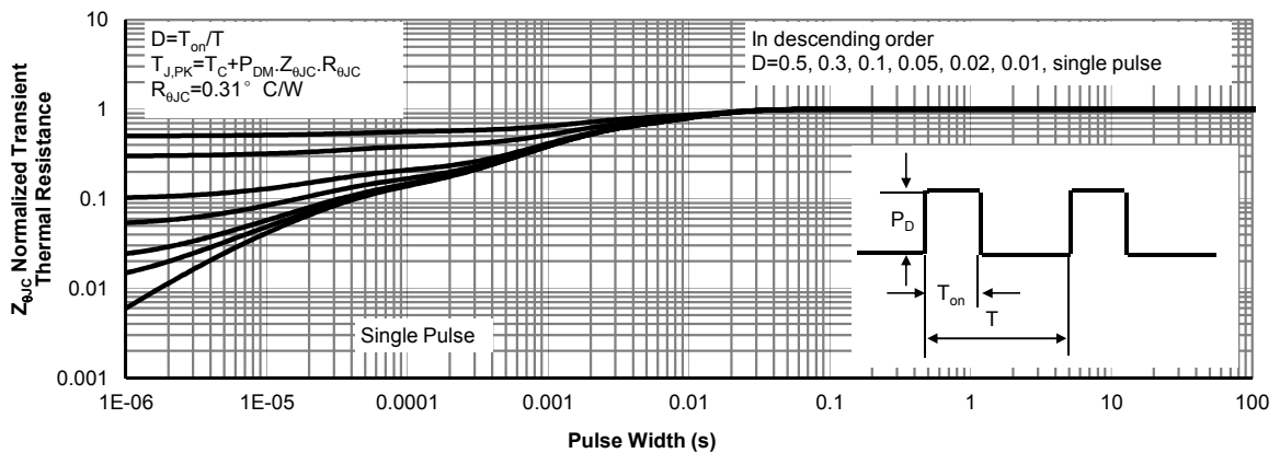
Figure 11: Normalized Maximum Transient Thermal Impedance for AOK10N90 (Note F)
