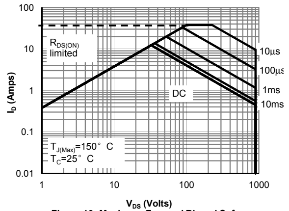
Figure 10: Maximum Forward Biased Safe Operating Area for AOK10N90 (Note F)
