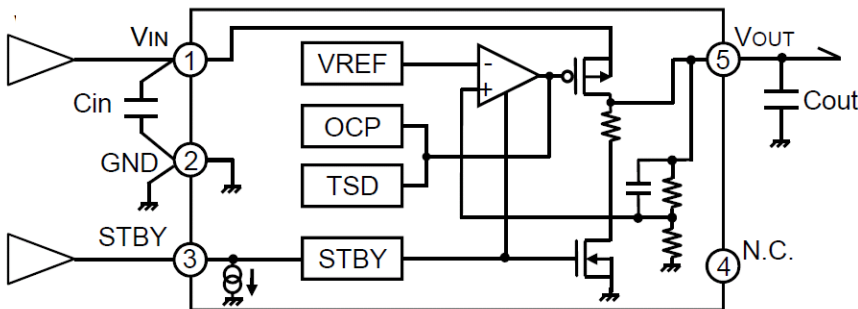
Figure 2. Block diagram
