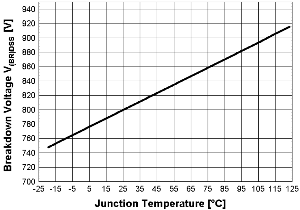
Figure 9 Drain-source breakdown voltage; V_{BR(DSS)} = f(T_j), I_D = 0.25mA
