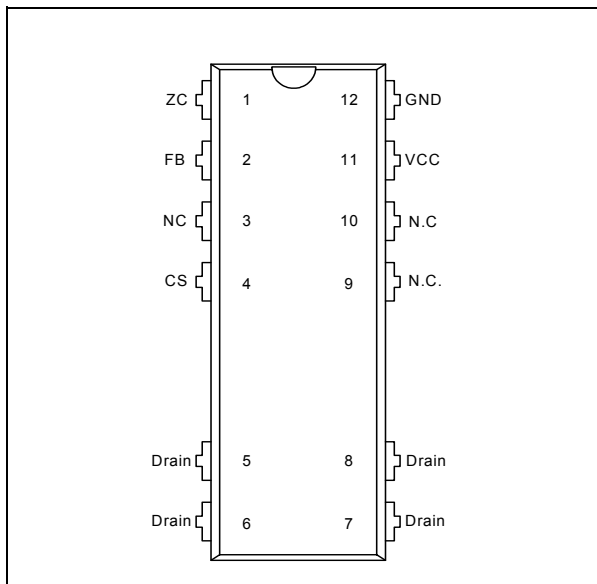
Figure 1 Pin Configuration PG-DSO-12 (top view)
