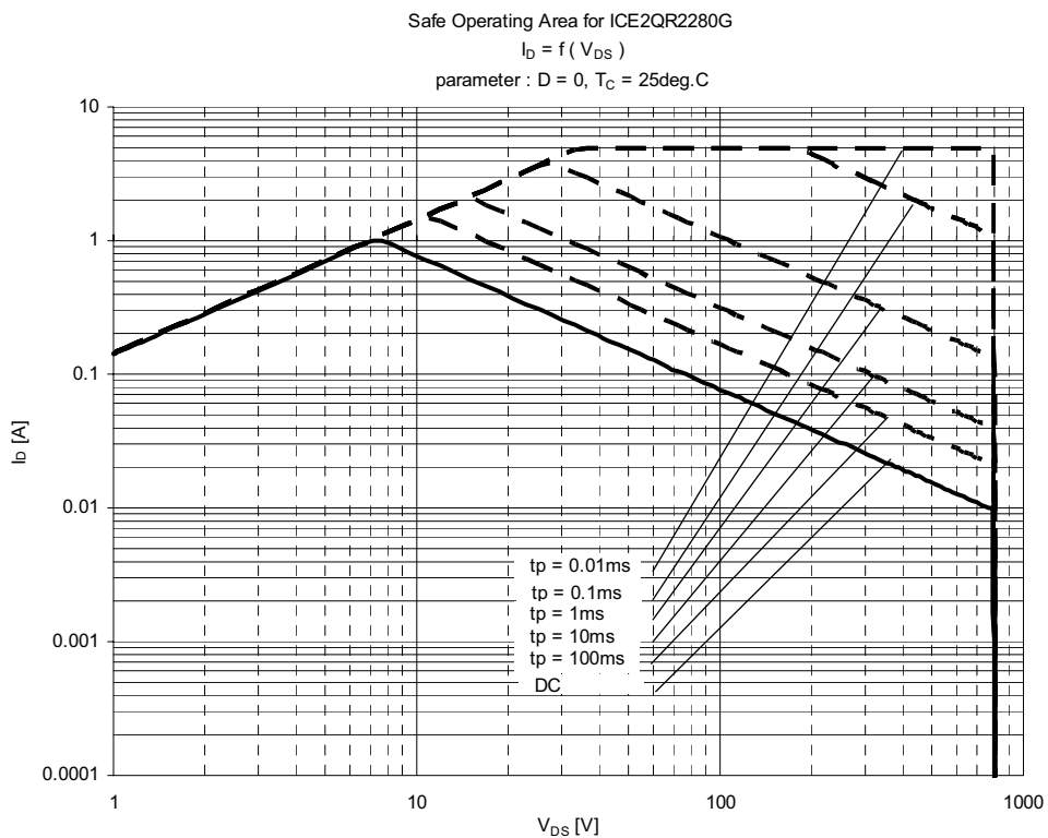
Figure 10 Safe Operating Area(SOA) curve for ICE2QR2280G
