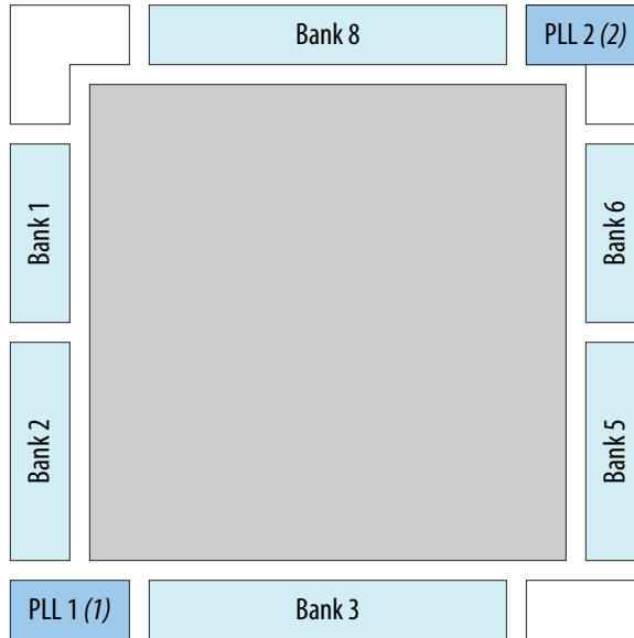
Figure 8. PLL Locations for 10M02 Device
