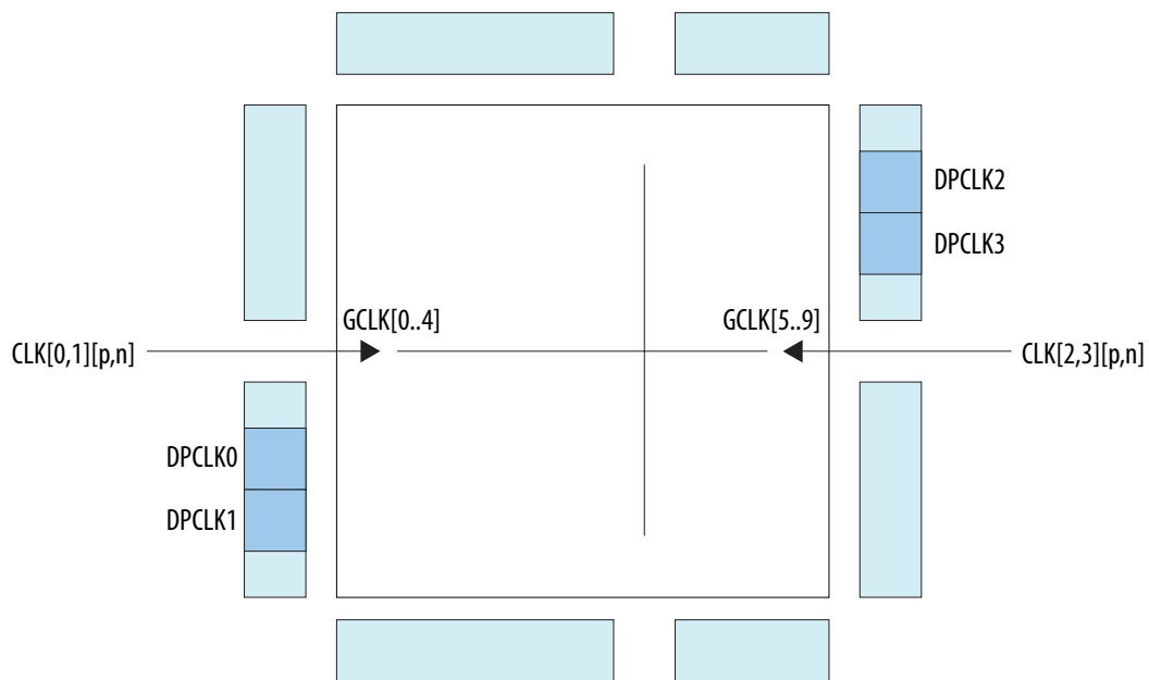
Figure 1. GCLK Network Sources for 10M02, 10M04, and 10M08 Devices
