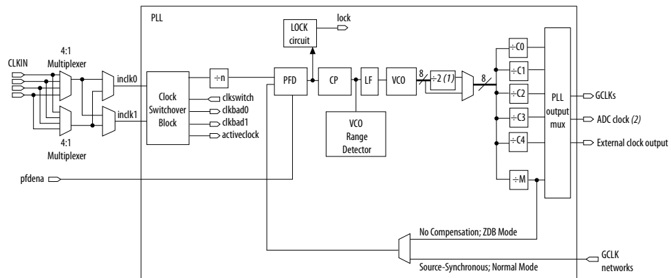
Figure 7. MAX 10 PLL High-Level Block Diagram
