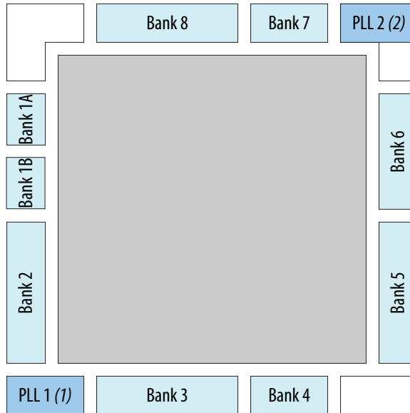
Figure 9. PLL Locations for 10M04 and 10M08 Devices
