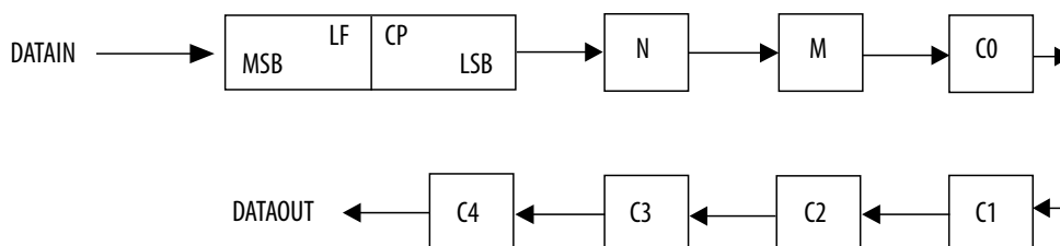
Figure 28. PLL Post-Scale Counter Scan Chain Bit Order
